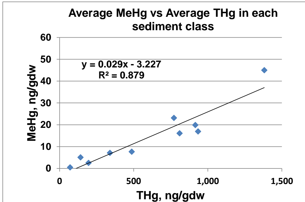
Figure 8-24. The average methyl Hg concentration in each sediment grab sample class vs the average total Hg concentration in each class.
