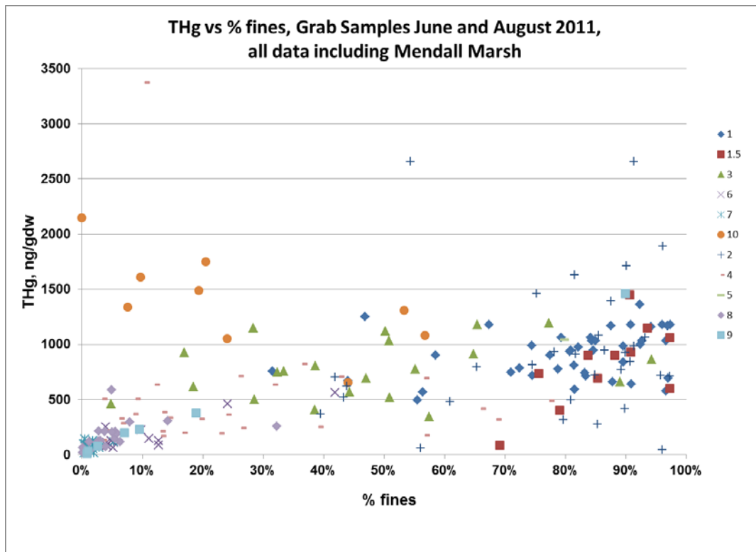
Figure 8-8. Total Hg plotted against % fines for all samples. Classes: 1 - unconsolidated mud, 1.5 - unconsolidated mud overlying consolidated mud, 2 - consolidated mud, 3 - mix of unconsolidated mud and anything else, 4 - mixed mud, sand, shells, rocks, woodchips, mussels, 5 - mussels with rocks etc., 6 - sand with mud, 7 - sand, 8 - sand with rocks, shells, woodchips, mussels, 9 - gravel or rocks; or scoured, 10 - woodchips.
