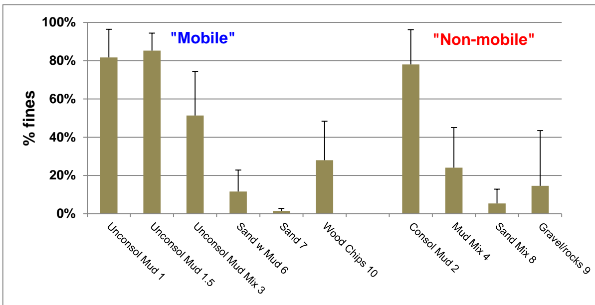
Figure 8-4. Average % fines in each class of grab sample, plus one standard deviation.
