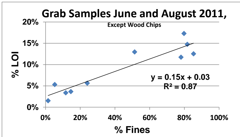
Figure 8-14. % LOI vs % fines each class of grab sample, except wood chips.
