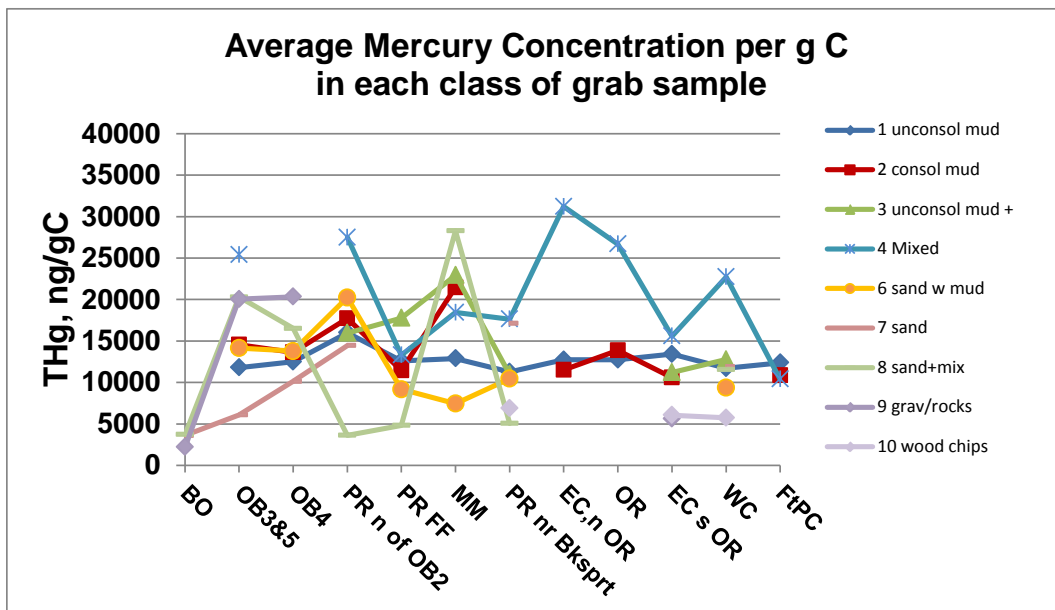
Figure 8-17b. Average total Hg concentration in each class of sediment, for each of the 12 geographic sub-areas, ordered north to south. Classes: 1 - unconsolidated mud, 1.5 - unconsolidated mud overlying consolidated mud, 2 - consolidated mud, 3 - mix of unconsolidated mud and anything else, 4 - mixed mud, sand, shells, rocks, woodchips, mussels, 5 - mussels with rocks etc., 6 - sand with mud, 7 - sand, 8 - sand with rocks, shells, woodchips, mussels, 9 - gravel or rocks; or scoured, 10 - woodchips.
