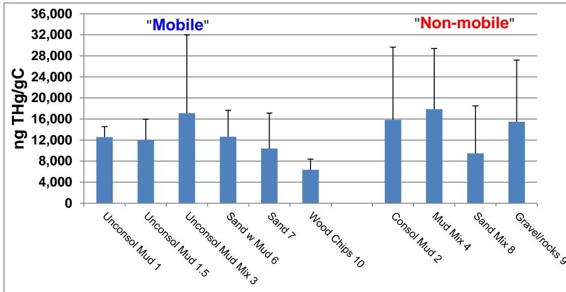
Figure 8-4. Average Hg concentrations, per gram carbon, in each class of grab sample, plus one standard deviation.
