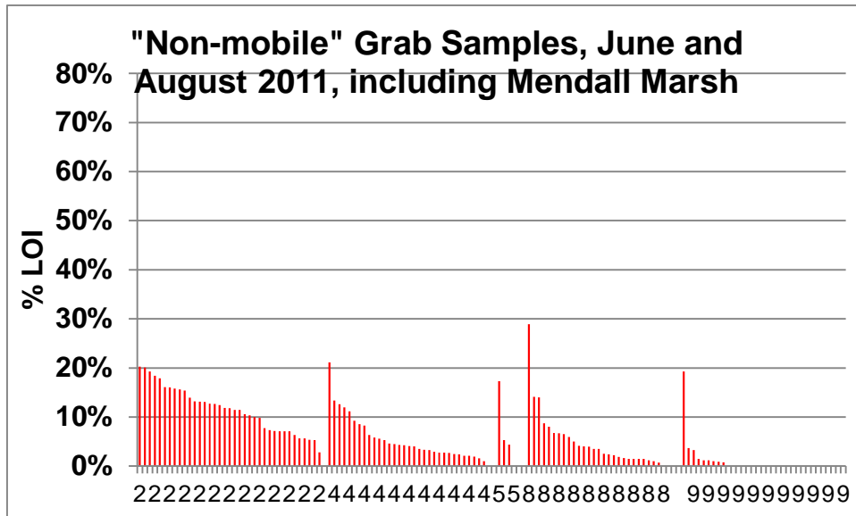
Figure 8-5b. Distribution of % LOI in each class of grab sample designated “non-mobile”. Classes: 2 - consolidated mud, and anything else, 4 - mixed mud, sand, shells, rocks, woodchips, mussels, 8 - sand with rocks, shells, woodchips, mussels, 9 - gravel or rocks; or scoured.
