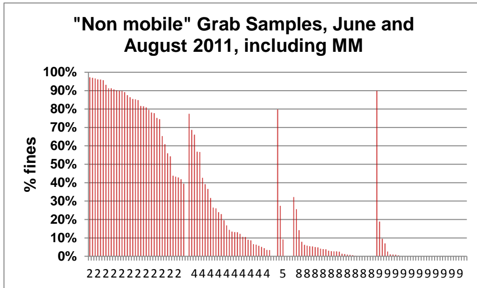
Figure 8-3b. Distribution of % fines in grab samples collected in June and August 2011 and designated “non-mobile”. Classes: 2 - consolidated mud, and anything else, 4 - mixed mud, sand, shells, rocks, woodchips, mussels, 8 - sand with rocks, shells, woodchips, mussels, 9 - gravel or rocks; or scoured. MM = Mendall Marsh.
