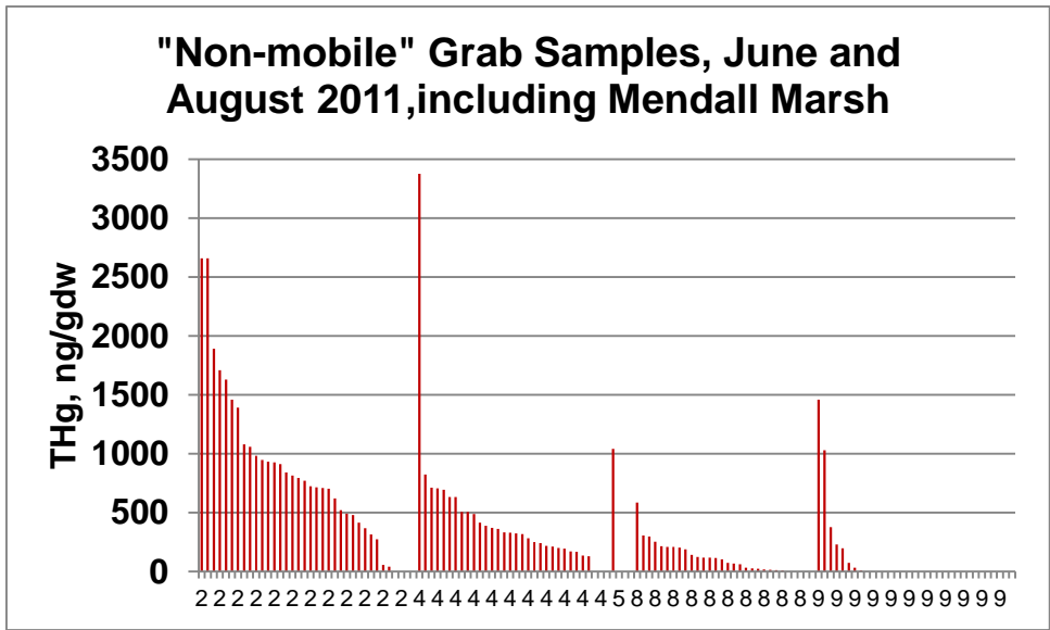
Figure 8-1b. Distribution of total Hg concentrations in grab samples collected in June and August 2011 and designated “non-mobile”. Classes: 2 - consolidated mud, 4 - mixed mud, sand, shells, rocks, woodchips, mussels, 5 - mussels with rocks and other material, 8 - sand with rocks, shells, woodchips, mussels, 9 - gravel or rocks; or scoured. Gaps in the graph indicate that a sample was taken in that category, but total Hg analysis was not done.
