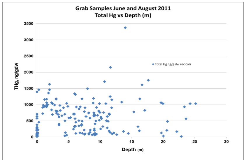
Figure 8-16a. Concentrations of total Hg in grab sediment samples plotted against depth of water at the sampling site.
