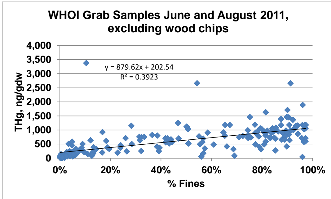
Figure 8-9. Total Hg concentrations plotted against % fines for all samples, excluding wood chips. Regression was significant at P < 0.001
