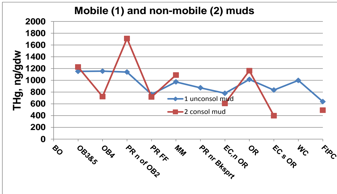
Figure 8-18a. Average total Hg concentration in “mobile and “non-mobile” classes of muds (1 and 2), for each geographic sub-area, ordered north to south.
