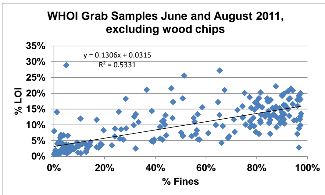
Figure 8-7. %LOI vs % fines in all grab samples except wood chips (wood chips were excluded because they are quite different in composition from all other sample types, and have very high % LOI and very low % fines). Regression was significant at P < 0.001 .
