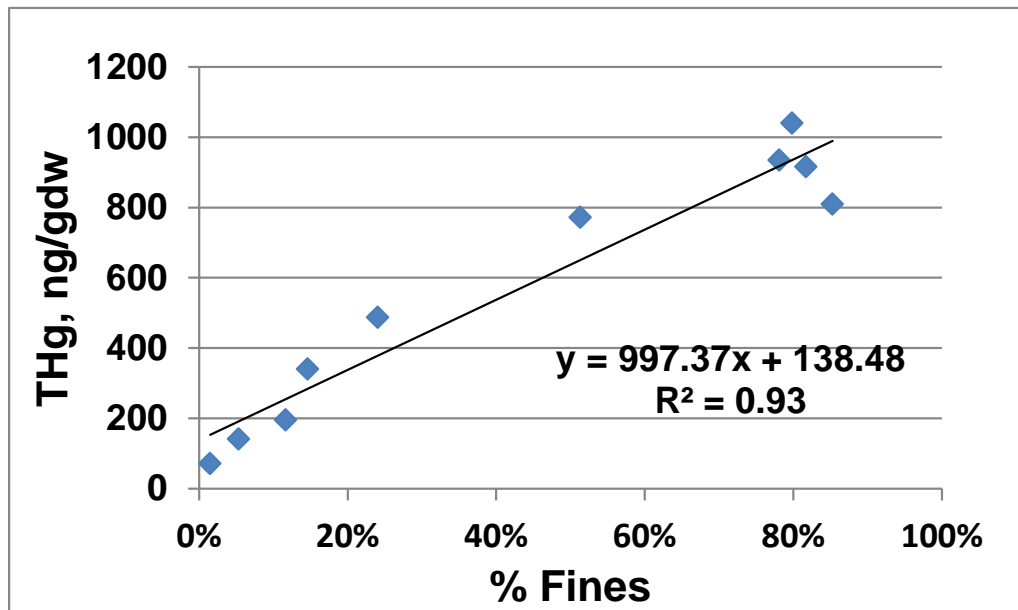
Figure 8-10. Average total Hg concentration for each class, plotted against average % fines for each class, excluding wood chips.
