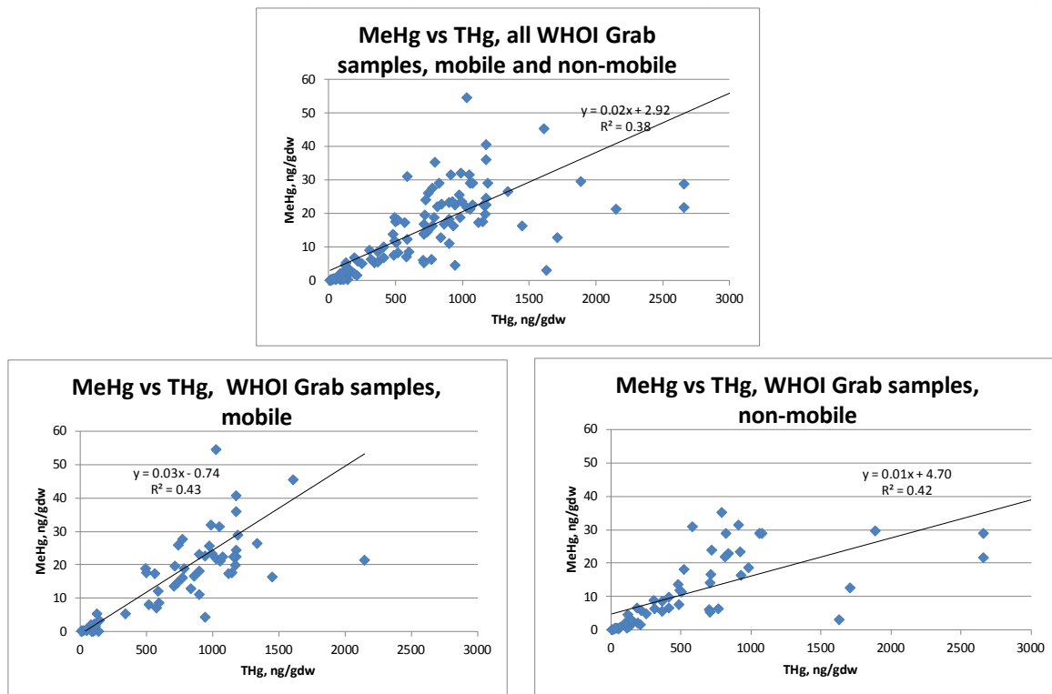
Figure 8-23. Methyl Hg vs total Hg in grab samples. All regressions were significant at the p < 0.005 level.
