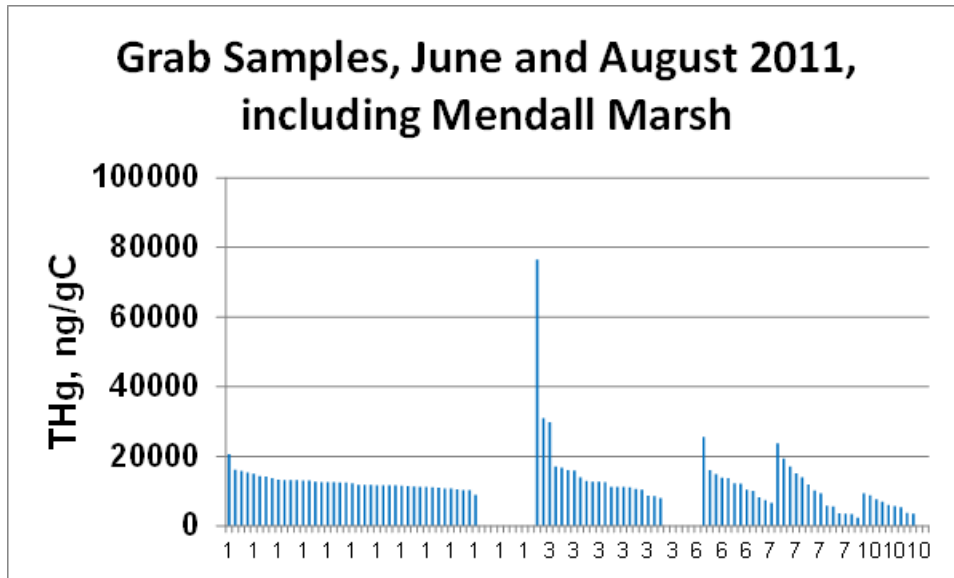
Figure 8-3a. Distribution of total Hg concentrations, per gram carbon, in grab samples collected in June and August 2011 and designated “mobile”. Classes: 1 - unconsolidated mud, 3 - mix of unconsolidated mud and other material, 6 - sand with mud, 7 - sand, 10 - woodchips. Gaps in the graph indicate that a sample was taken in that category, but total Hg analysis was not done.
