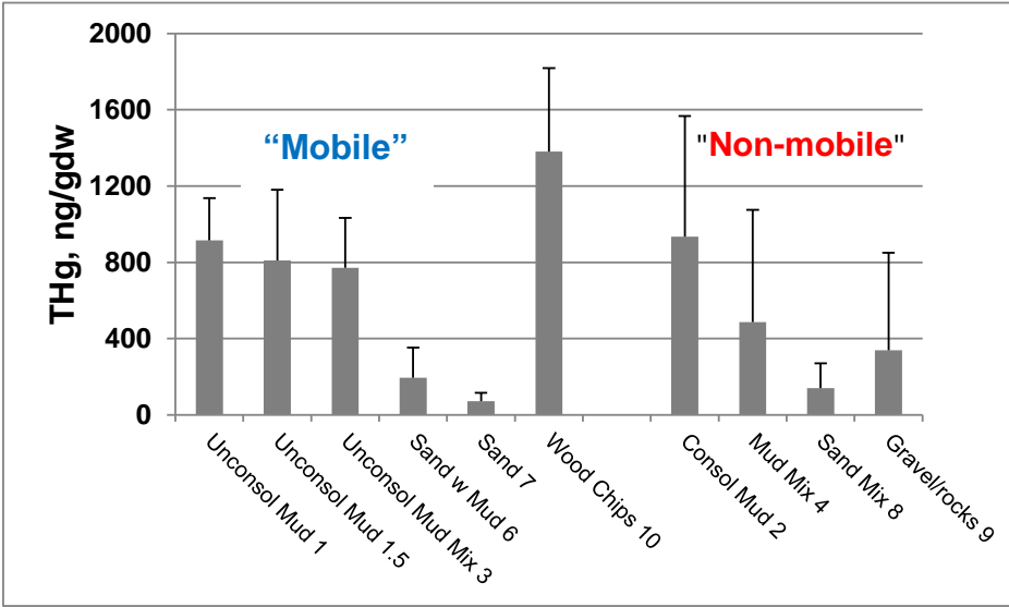
Figure 8-2. Average Hg concentrations in each class of grab sample, plus one standard deviation.
