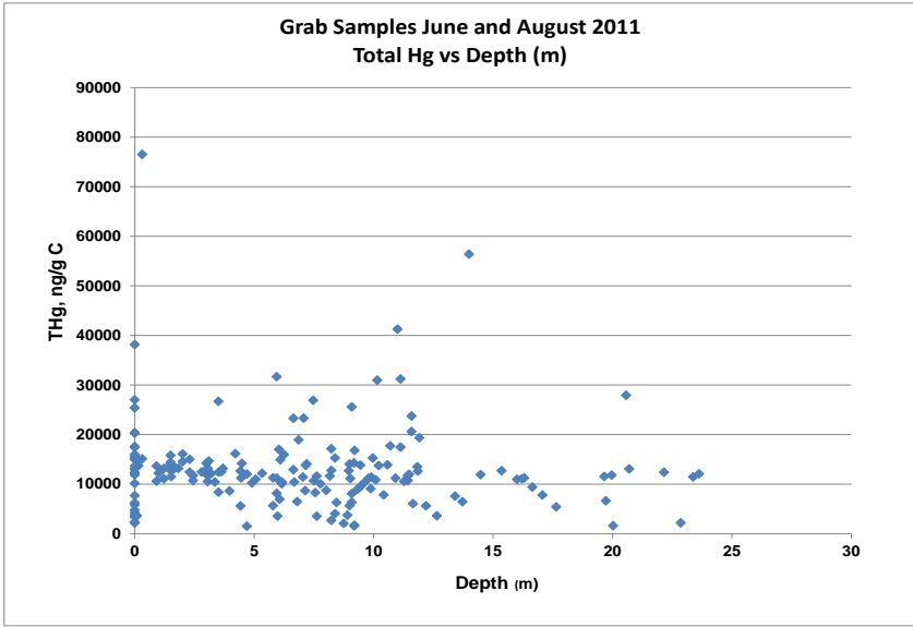
Figure 8-16b. Hg concentrations per gram carbon vs depth in the main stem of the Penobscot River.
