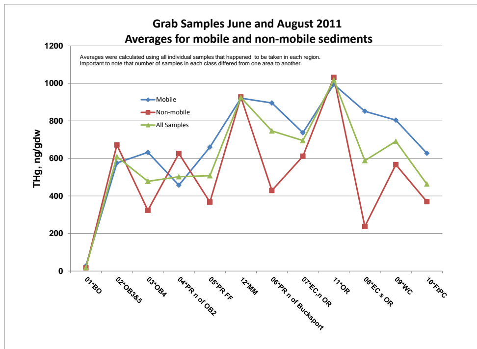
Figure 8-20. Average total Hg concentrations in mobile and non-mobile sediments, for each geographic sub-area, ordered roughly north to south.
