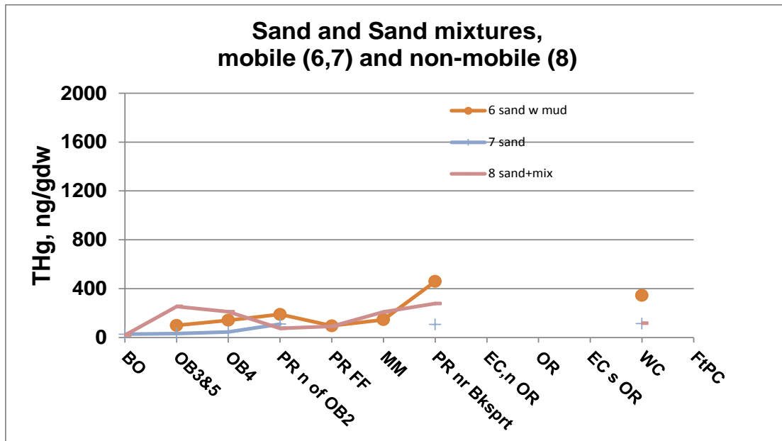
Figure 8-19a. Total Hg concentrations in “mobile” and “non-mobile” sand and sand mixtures. Mobile classes: 6 - sand with mud, 7 - sand. Non-mobile class: 8 - sand with rocks, shells, woodchips, mussels.
