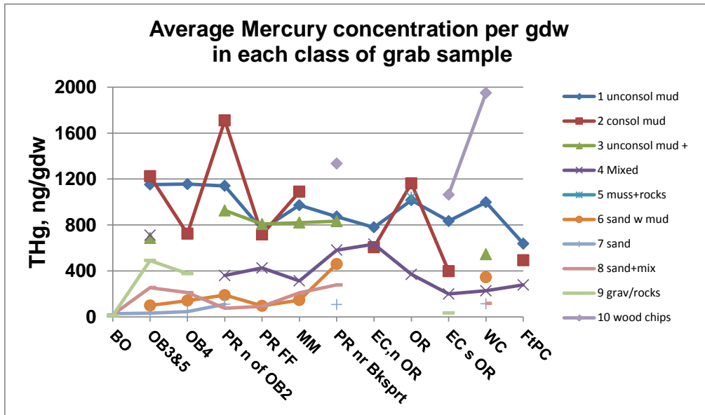
Figure 8-17a. Average total Hg concentration in each class of sediment, for each of the 12 geographic sub-areas, ordered north to south. Classes: 1 - unconsolidated mud, 1.5 - unconsolidated mud overlying consolidated mud, 2 - consolidated mud, 3 - mix of unconsolidated mud and anything else, 4 - mixed mud, sand, shells, rocks, woodchips, mussels, 5 - mussels with rocks etc., 6 - sand with mud, 7 - sand, 8 - sand with rocks, shells, woodchips, mussels, 9 - gravel or rocks; or scoured, 10 - woodchips.
