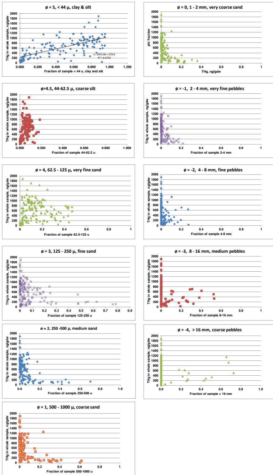
Figure 8-11. Abundance of each grain size fraction in samples of different Hg concentrations. Hg concentrations were measured on whole sediment, and grain size fractions were measured on a separate aliquot of the same sample.
