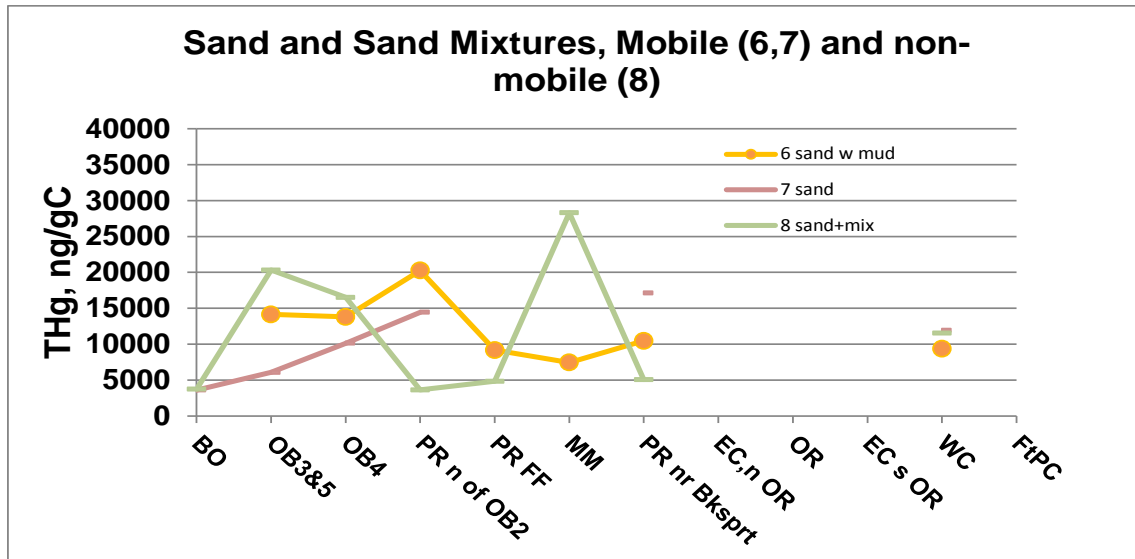
Figure 8-19b. Total Hg concentrations per unit of carbon in “mobile” and “non-mobile” sand and sand mixtures. Mobile classes: 6 - sand with mud, 7 - sand. Non-mobile class: 8 - sand with rocks, shells, woodchips, mussels.
