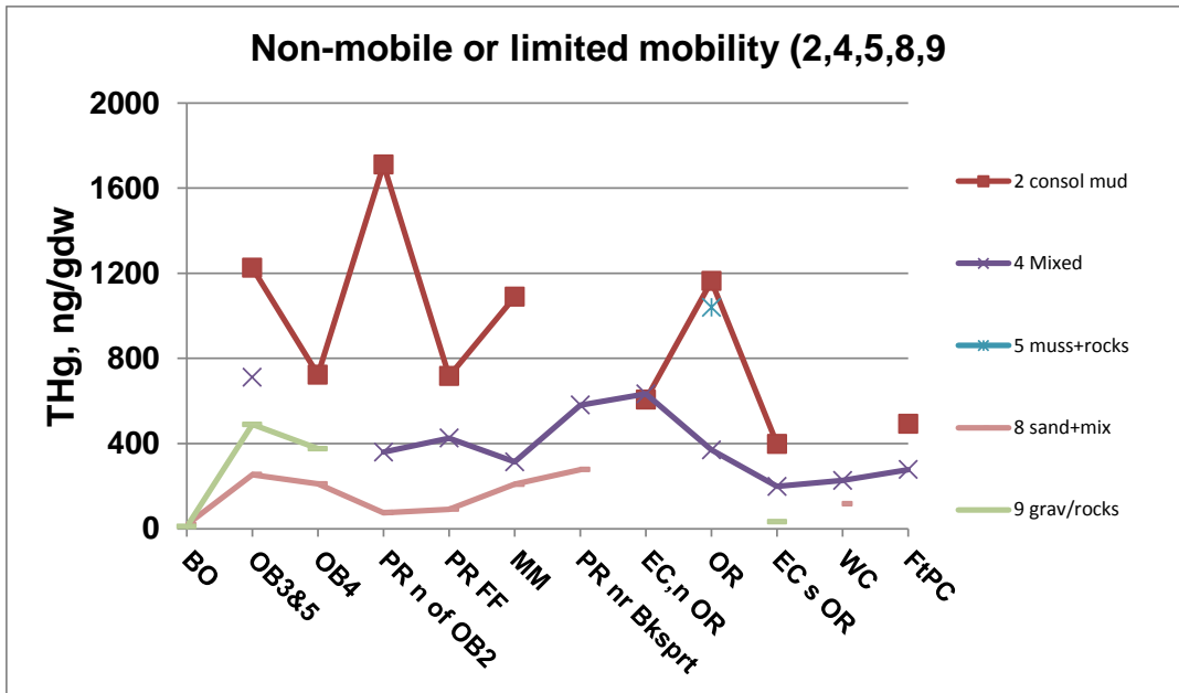
Figure 8-22. Total Hg concentrations in the “non-mobile” classes of sediments: 2 - consolidated mud, 4 - mixed mud, sand, shells, rocks, woodchips, mussels, 5 - mussels with rocks etc., 6 - sand with mud, 8 - sand with rocks, shells, woodchips, mussels, 9 - gravel or rocks; or scoured.
