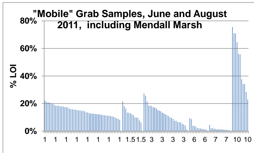
Figure 8-5a. Distribution of % LOI each class of grab sample designated "mobile". Classes: 1 - unconsolidated mud, 3 - mix of unconsolidated mud and anything else, 6 - sand with mud, 7 - sand, 10 - woodchips.
