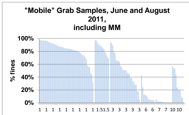
Figure 8-3a. Distribution of % fines in grab samples collected in June and August 2011 and designated “mobile”. Classes: 1 - unconsolidated mud, 3 - mix of unconsolidated mud and anything else, 6 - sand with mud, 7 - sand, 10 - woodchips.
