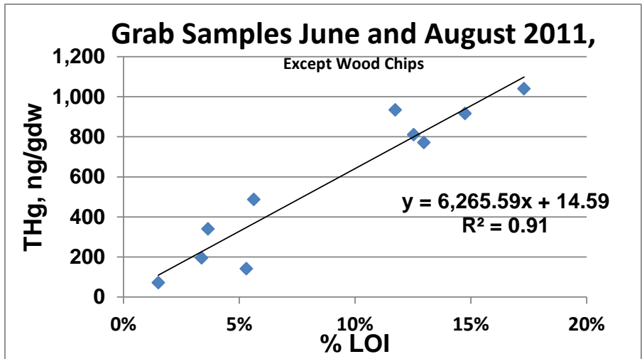
Figure 8-13. Average total Hg concentrations vs average % LOI in each class of grab sample, except wood chips.
