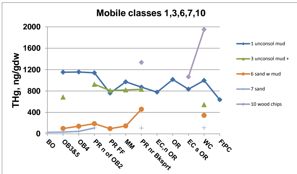
Figure 8-21. Total Hg concentrations in the “mobile” classes of sediments: 1 - unconsolidated mud, 1.5 - unconsolidated mud overlying consolidated mud, 3 - mix of unconsolidated mud and anything else, 6 - sand with mud, 7 - sand, 10 - woodchips.
