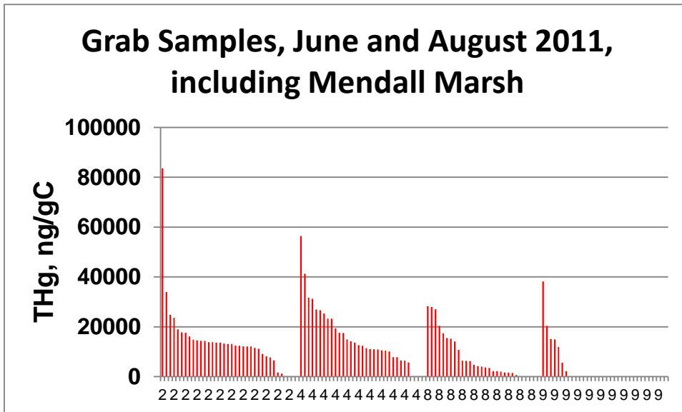
Figure 8-3b. Distribution of total Hg concentrations, per gram carbon, in grab samples collected in June and August 2011 and designated “non-mobile”. Classes: 2 - consolidated mud, 4 - mixed mud, sand, shells, rocks, woodchips, mussels, 8 - sand with rocks, shells, woodchips, mussels, 9 - gravel or rocks; or scoured. Gaps in the graph indicate that a sample was taken in that category, but total Hg analysis was not done.
