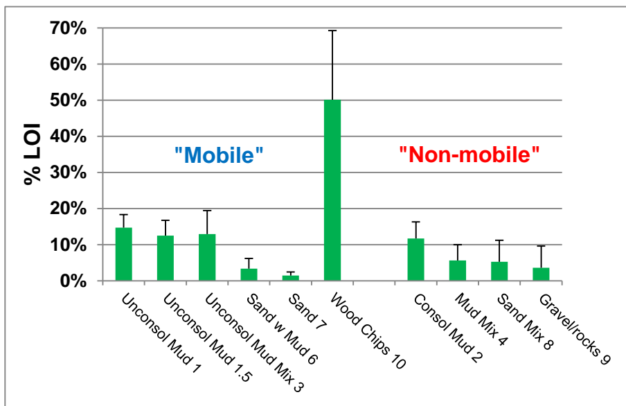
Figure 8-6. Average % LOI in each class of grab sample, plus one standard deviation.
