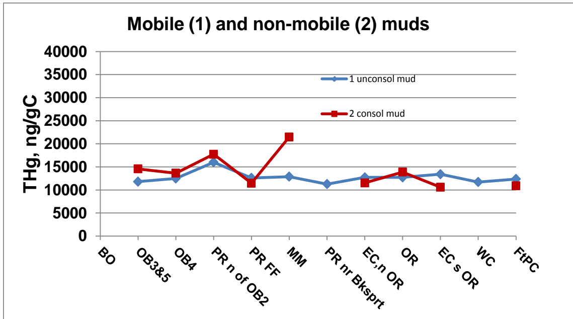
Figure 8-18b. Average total Hg concentration per unit carbon in “mobile and “non-mobile” classes of muds (1 and 2), for each geographic sub-area, ordered north to south.
