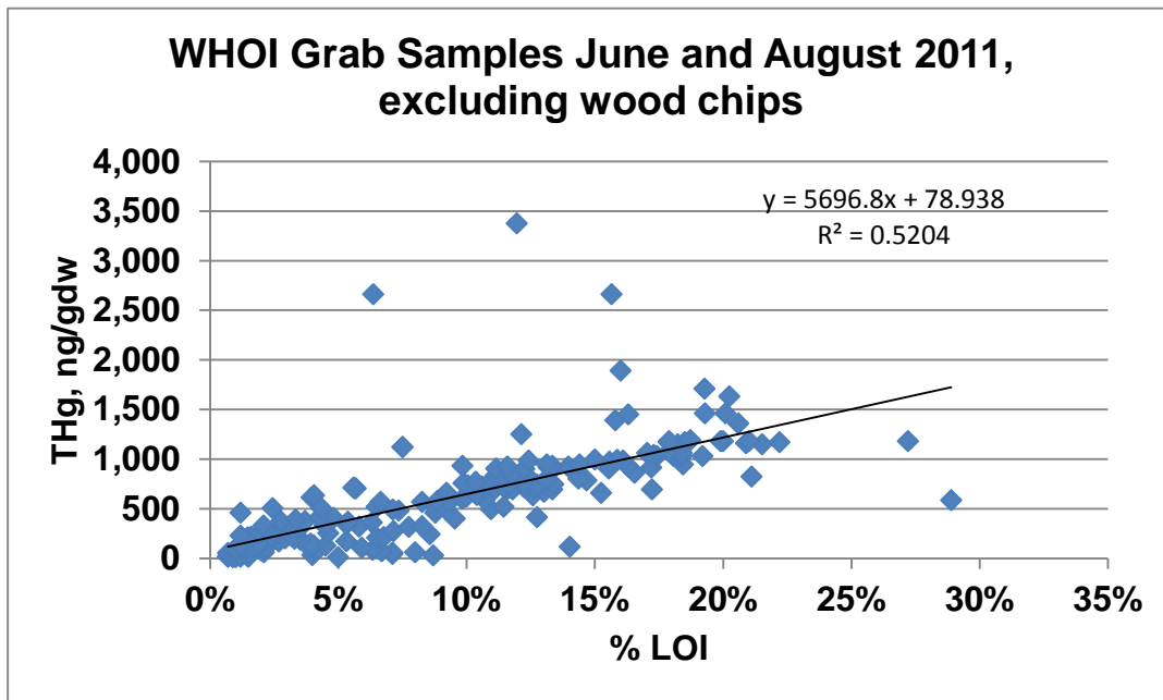
Figure 8-12. Total Hg vs Loss on Ignition in all grab samples except wood chips. Regression was significant at P < 0.001
