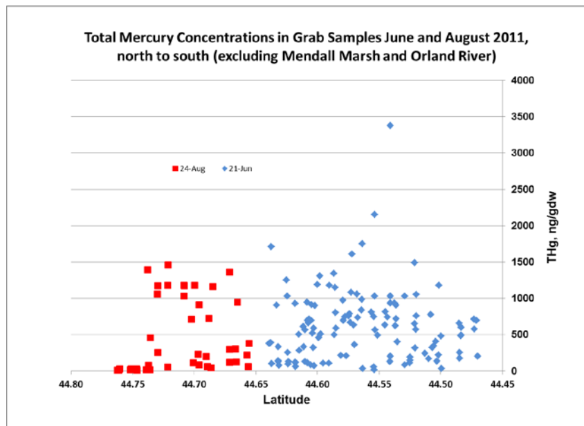
Figure 8-15a. Concentrations of total Hg in sediment samples from the main stem of the Penobscot River from Brewer to Fort Point Cove, plotted on a north to south gradient.
