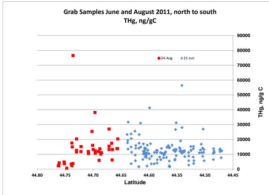
Figure 8-15b. The north to south pattern of concentrations of total Hg per unit of carbon (estimated using % LOI measurements and assuming 50% of the LOI was due to carbon).
