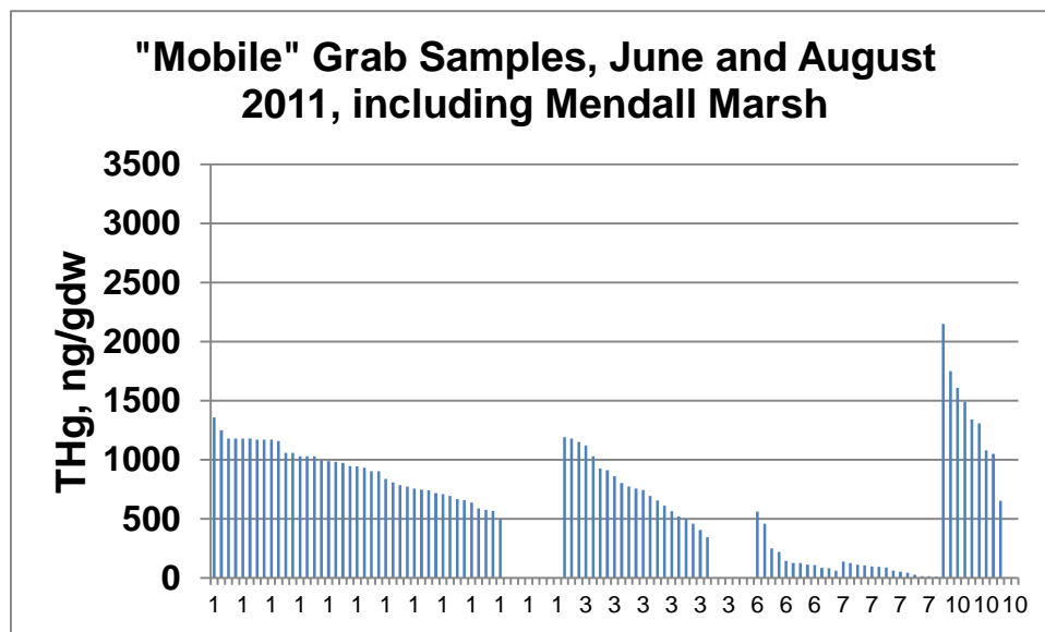
Figure 8-1a. Distribution of total Hg concentrations in grab samples collected in June and August 2011 and designated "mobile". Classes: 1 - unconsolidated mud, 3 - mix of unconsolidated mud and other material, 6 - sand with mud, 7 - sand, 10 - woodchips. Gaps in the graph indicate that a sample was taken in that category, but total Hg analysis was not done.
